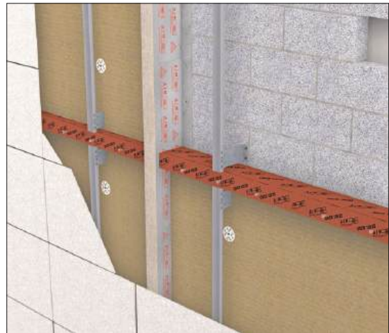
Masonry construction substrate
