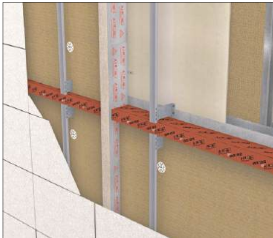
Steel Frame / SFS construction substrate
